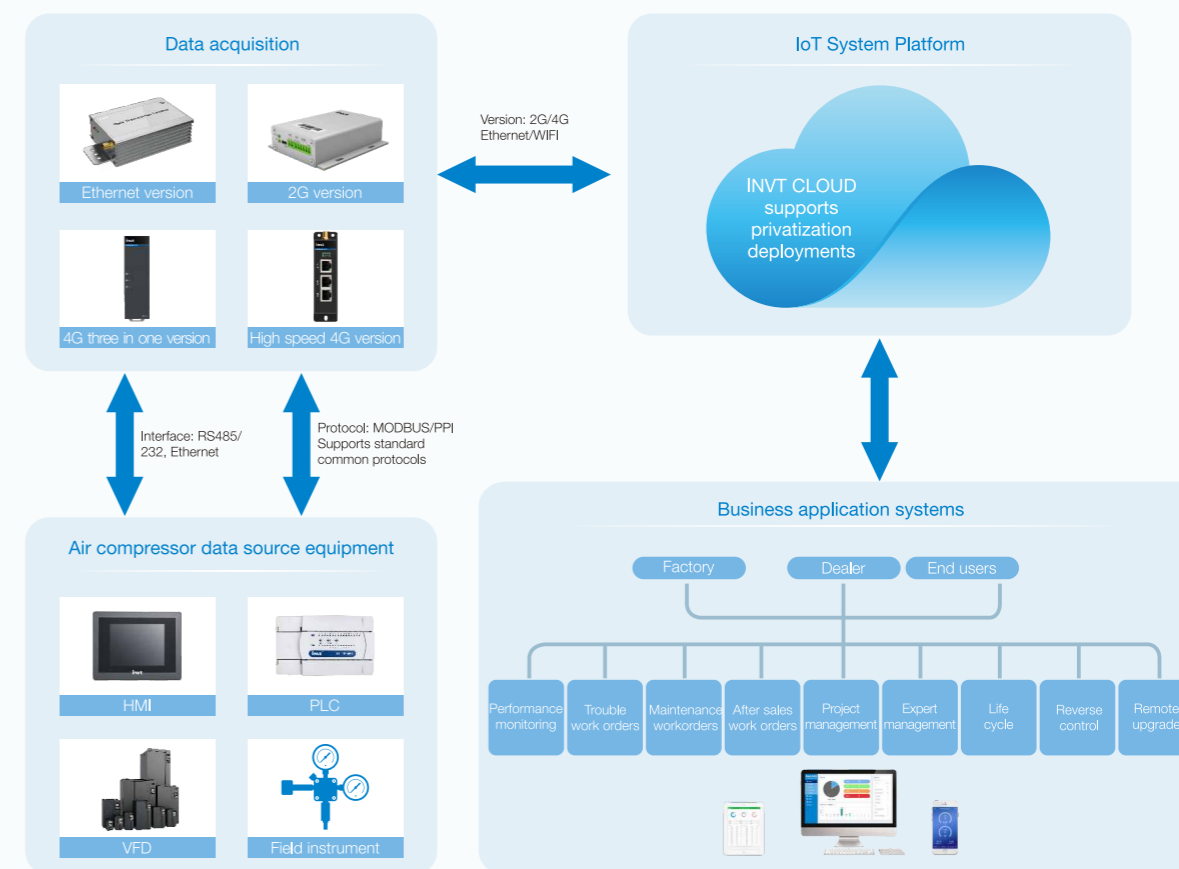
INVT IoT architecture diagram
